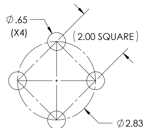
Recommended Mounting Holes
